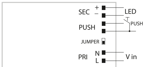
PUSH diagram - Collegamento PUSH
