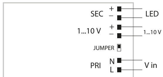
1...10 V diagram - Collegamento 1...10 V
